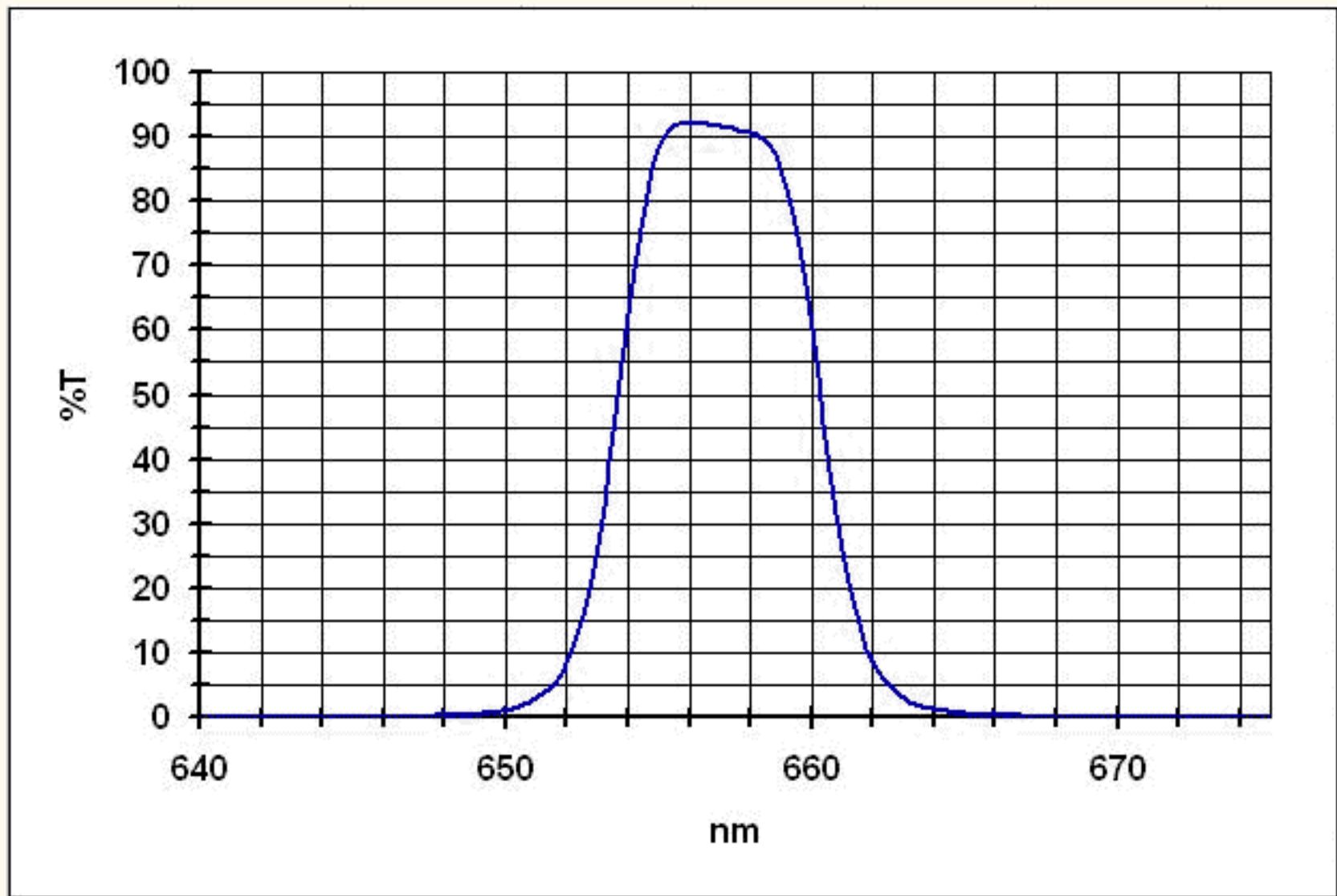
Baader H-Alpha Passfilter (FHALN) Filter Curve, Expanded Scale
